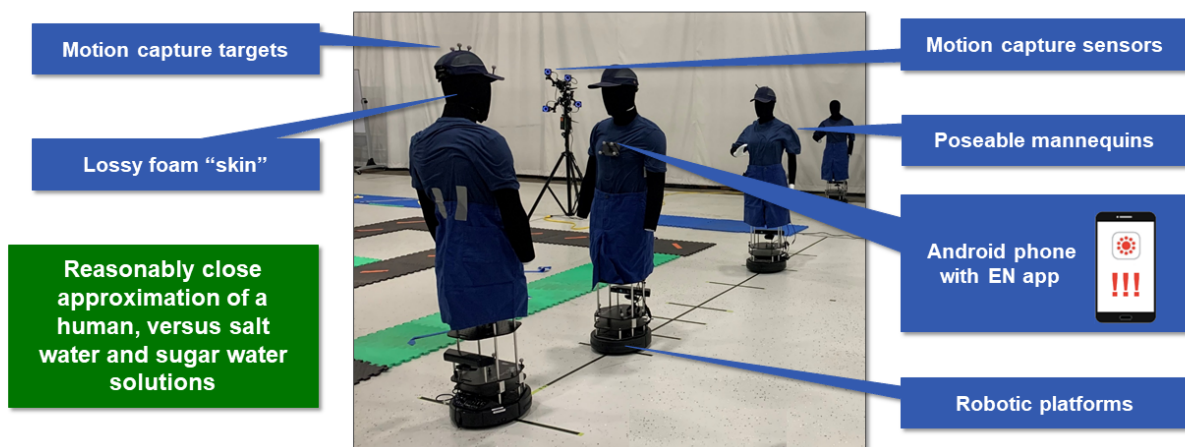
Figure 3: Data collection hardware, software, and infrastructure in the ASDF.
