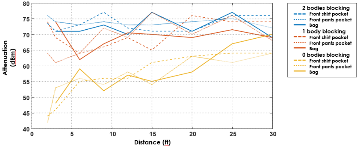
Figure 5: Attenuation vs actual distance in large indoor space.
